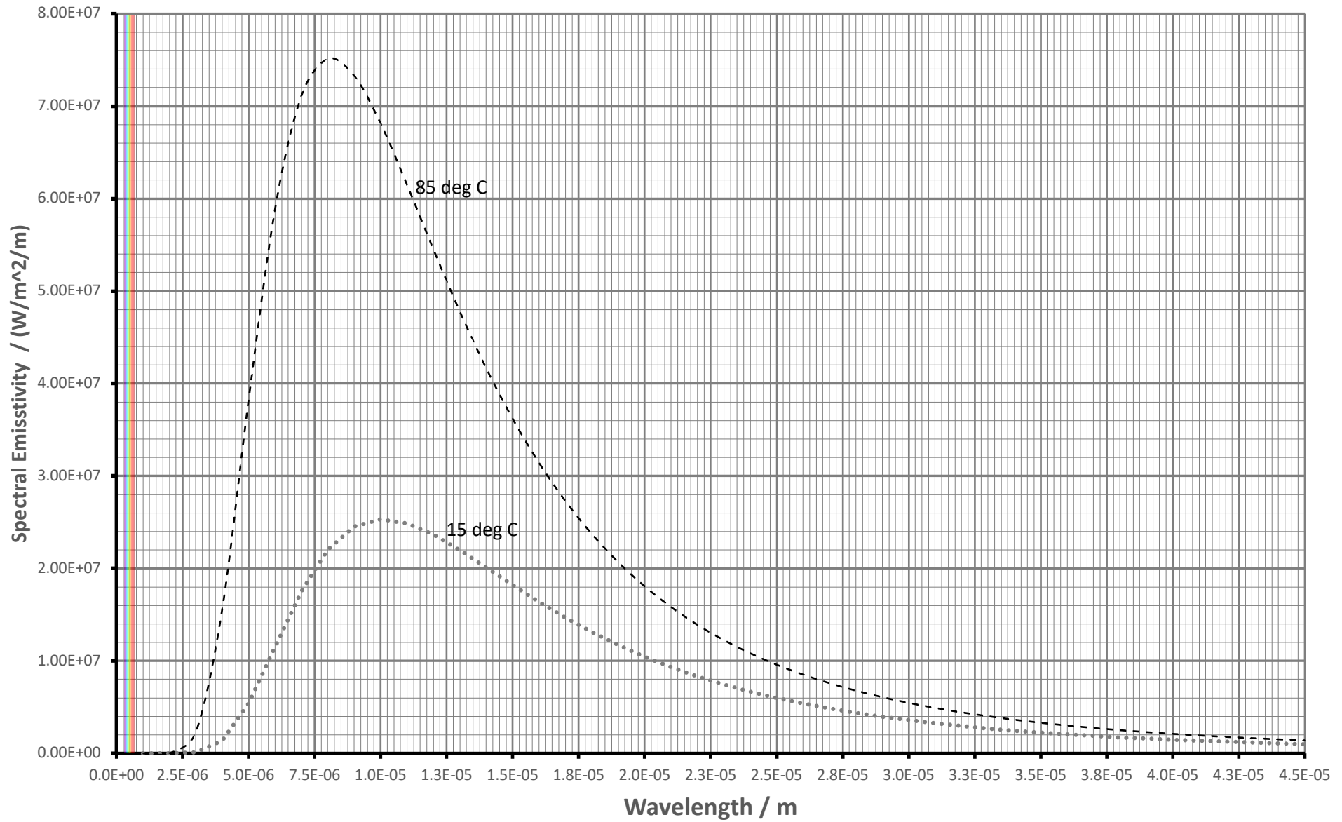
Power output against wavelength for two blackbodies in thermal equilibrium with their surroundings at 15 and 85 degrees Celsius
